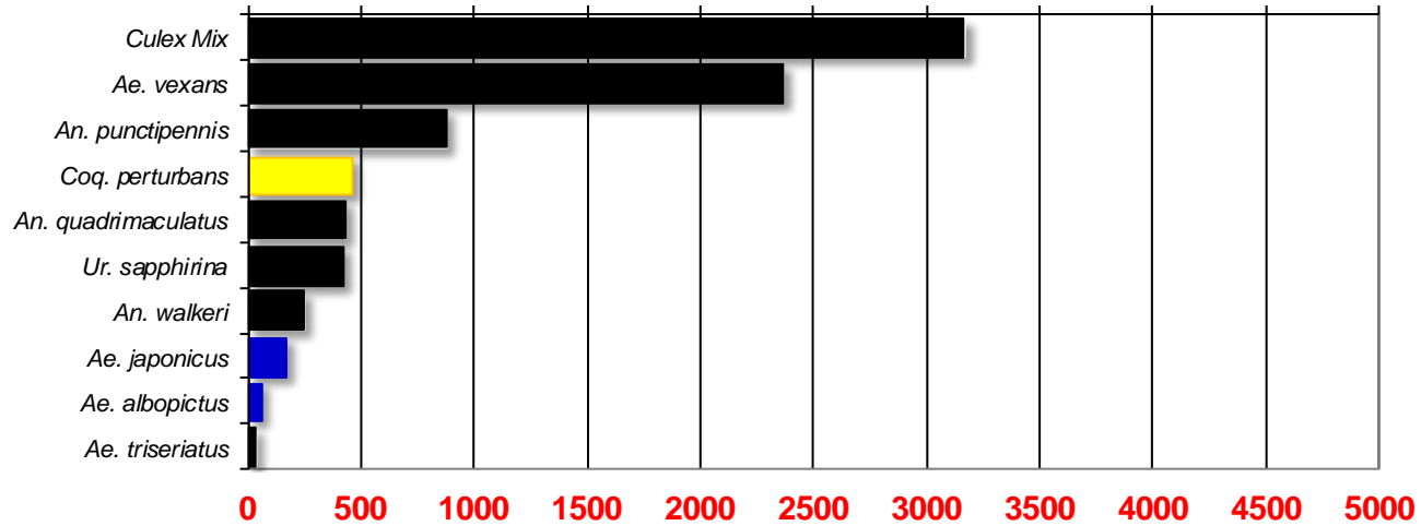
Total # mosquitoes
