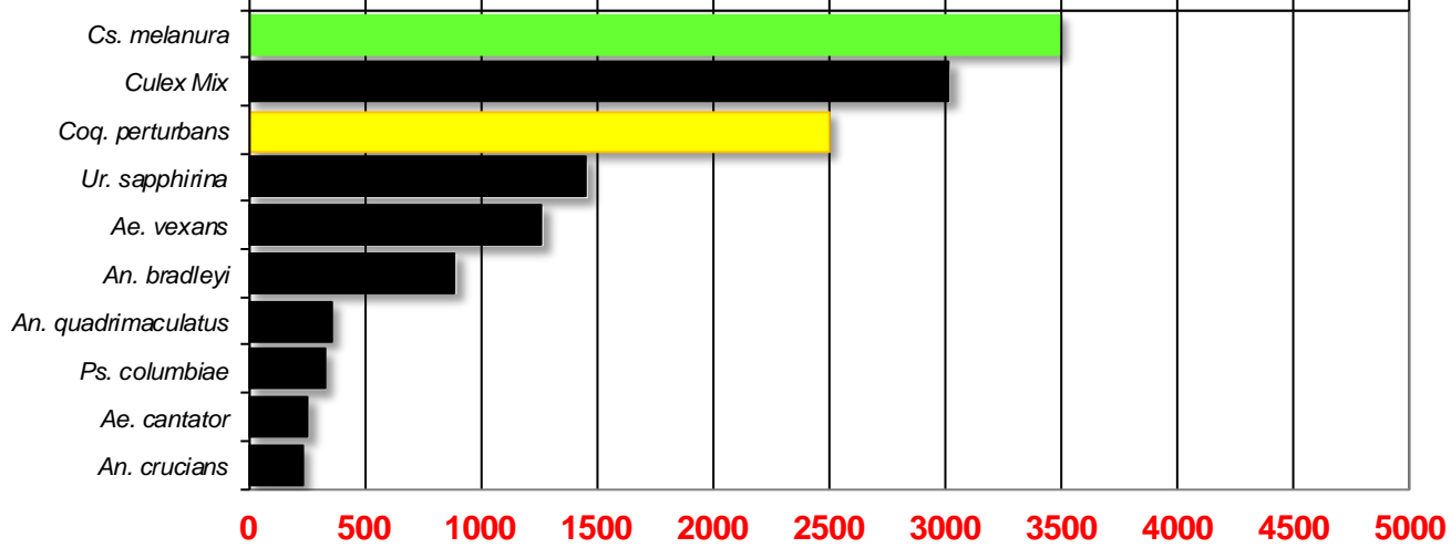
Total # mosquitoes
