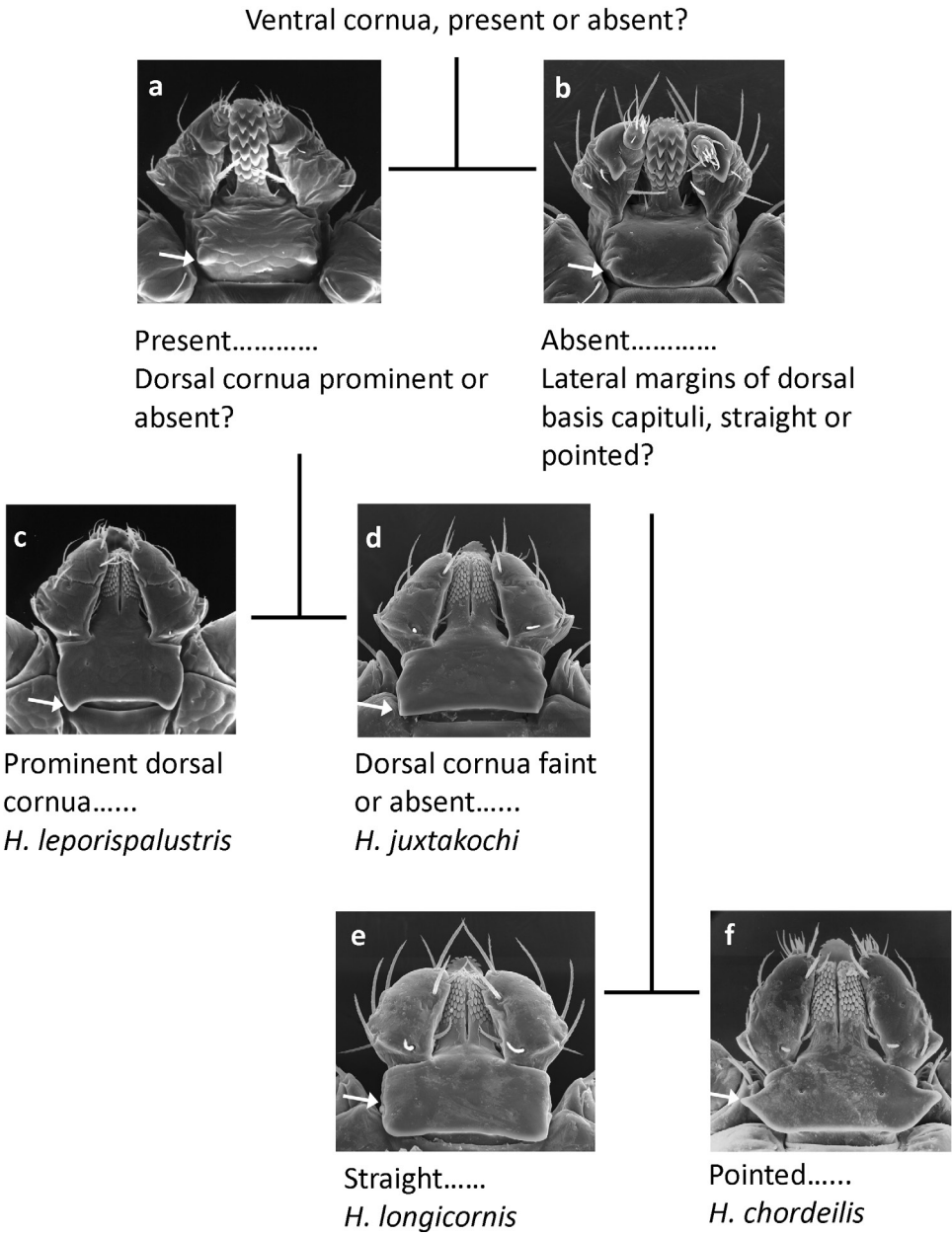
Figure 7. Pictorial key to larvae of Haemaphysalis spp. occurring in North America.
