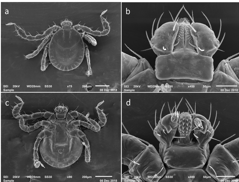
Figure 4. SEM photos of larval H. longicornis from a colony started with specimens from Queensland, Australia (Accession # RML58949). a dorsal full body b dorsal capitulum c ventral full body d ventral capitulum.
