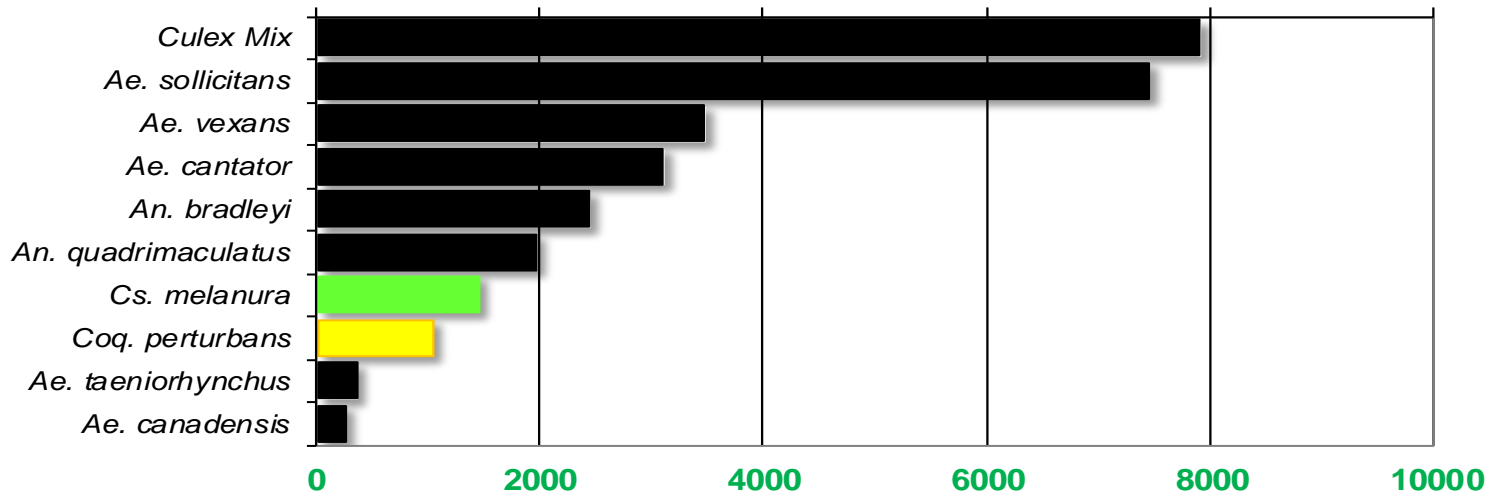
Total # mosquitoes
