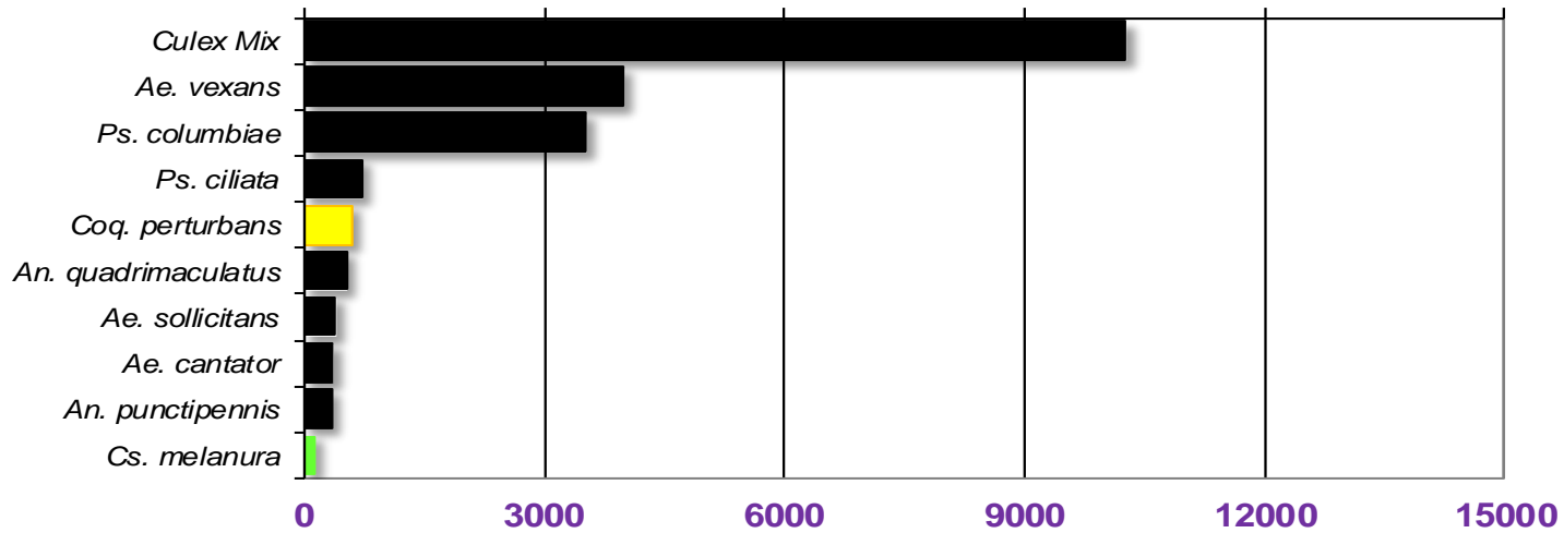
Total # mosquitoes
